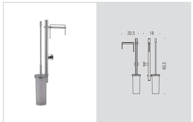
W4923 Colonna con porta rotolo e porta scopino Column equipped with paper holder and brush holder
