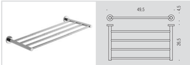
W4987 Rack porta salvietta Rack towel holder
