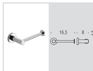
W4908 Porta rotolo reversibile Reversible paper holder
