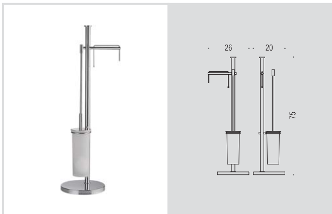
W4935 Piantana con porta rotolo e porta scopino Standing column equipped with paper holder and brush holder
